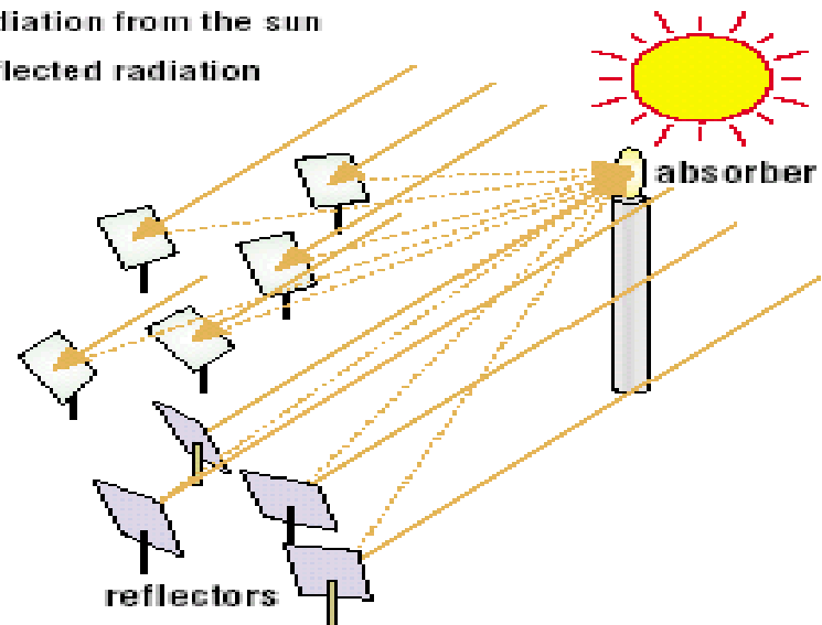
Solar tower CST (Point concentrating type)
